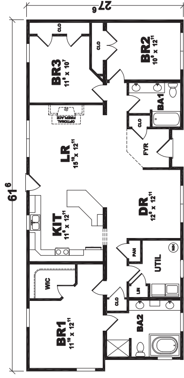
First Floor Layout
