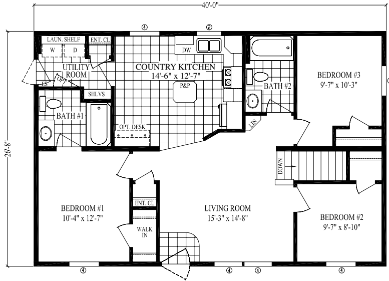
4428-401 1173 Sq. Ft.
