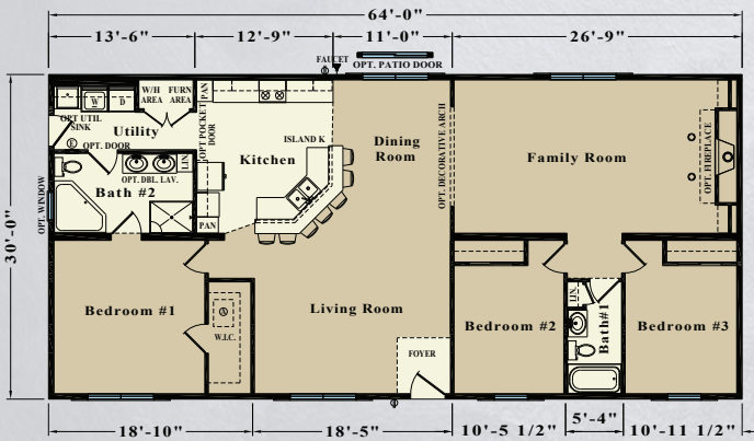
MODEL JR22A - 1,920 S.F.
