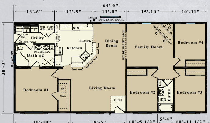
MODEL JR22B - 1,920 S.F.
