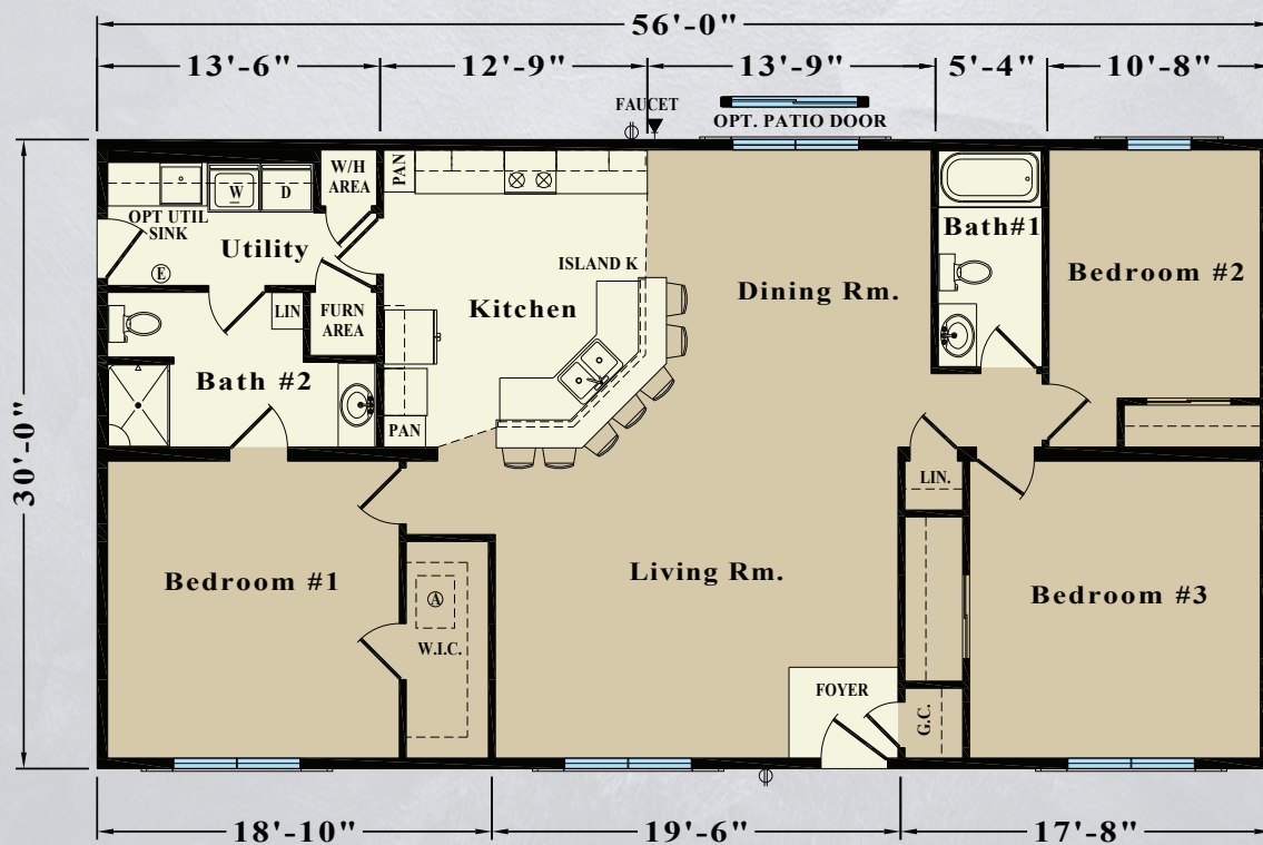
MODEL JR22C - 1,680 S.F.
