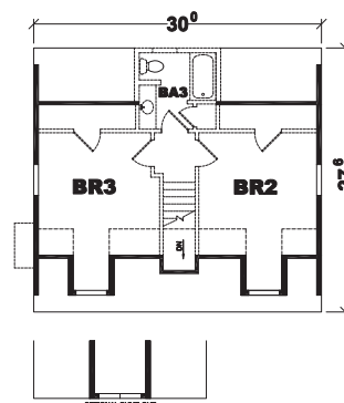
Proposed Second Floor Layout
